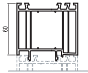
140207 - (EX60WF2) EXTENSION FRAME 60mm
