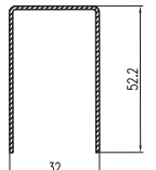
209004 - (STU32x52.2x1.2)
