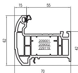
100015 - (PV62WF) FLY MULLION
