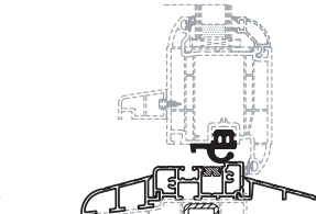
THRESHOLD AND CILL RAMP
