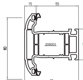
100013 - (TM80WF) INTERMEDIATE 'T' TRANSOM/MULLION
