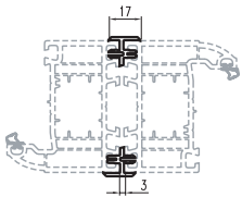
120224 - (CP17) COUPLING SINGLE SIDED
