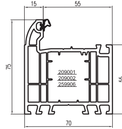
100004 - (OF75WF) LARGE OUTERFRAME
