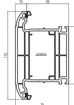
100010 - (TM115WF) DOOR MIDRAIL & LARGE TRANSOM/MULLION
