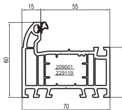
100003 - (OF60WF) INTERMEDIATE OUTERFRAME
