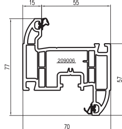
100007 - (SA77WF) TILT & TURN SASH
