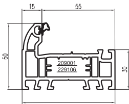
100002 - (OF50WF) SLIM OUTERFRAME
