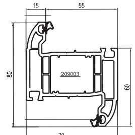
100014 - (ZM80WF) INTERMEDIATE 'T' TRANSOM/MULLION
