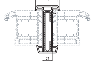
140218 - (CP48x70) COUPLING SLEEVE PROFILE 229018 - (STC13x80x2) REINFORCEMENT
