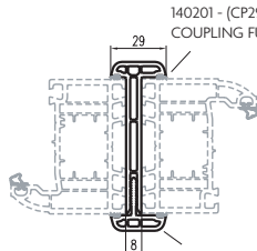
140201 - (CP29x70F) COUPLING FULL WIDTH 70mm FEMALE
