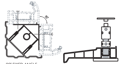
BAY CONNECTOR LOAD BEARING JACK ASSEMBLY
