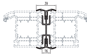
V MULTI COUPLER VARIABLE ANGLE INTERVAL COVER
