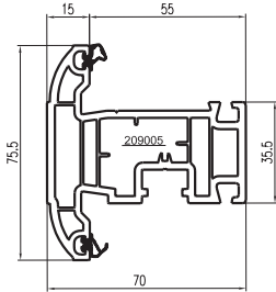
100005 - (SA75WF) INTERNAL GLAZED CASEMENT SASH
