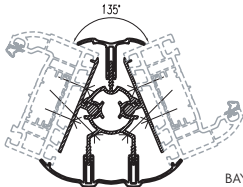
VARIABLE ANGLE BAY ASSEMBLY (135° SHOWN)
