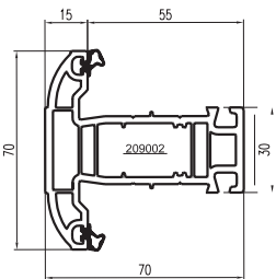
100011 - (TM70WF) SLIM 'T' TRANSOM/MULLION
